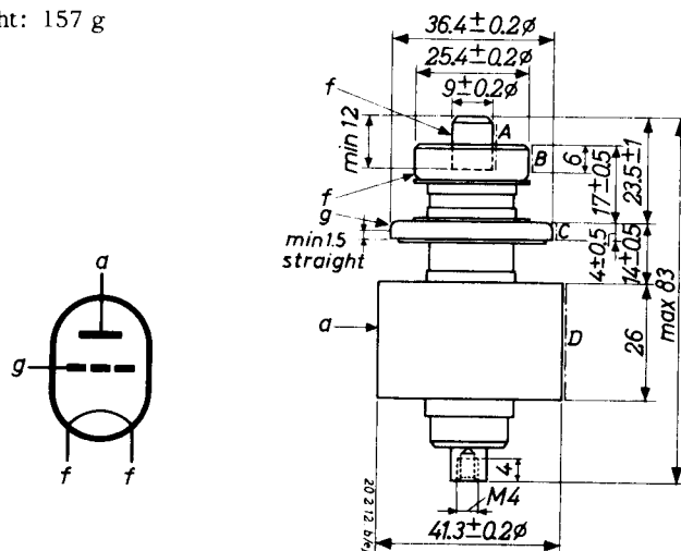
Fig. 1 Mechanical outline.
