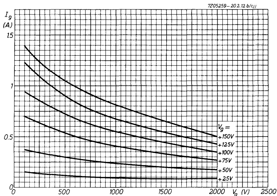
Fig. 3 I_g/V_a characteristics.
