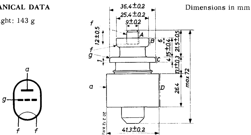
Fig. 1 Mechanical outline.
