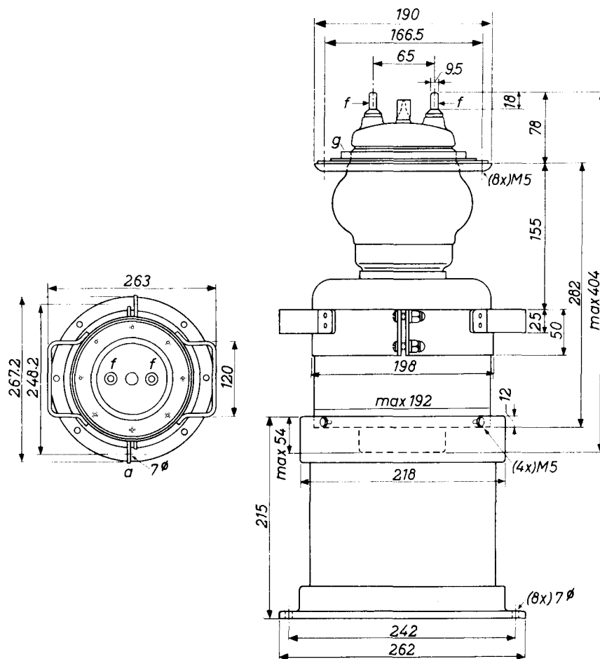
Fig. 2 Mechanical outline.
