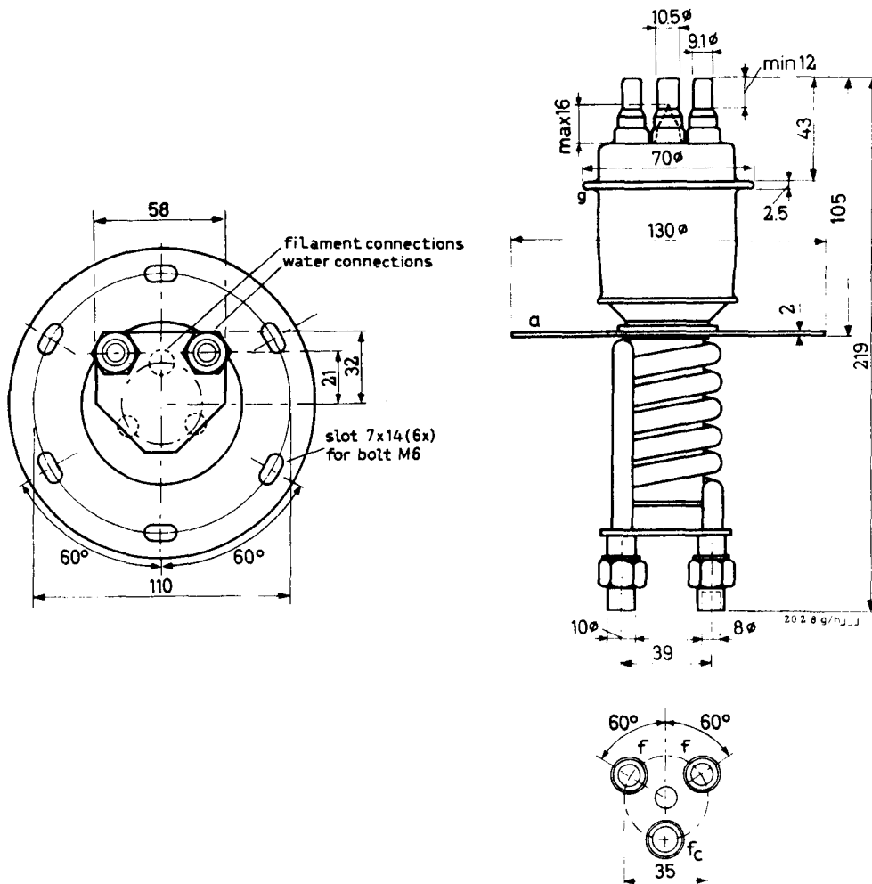
Fig. 1 Mechanical outline.
