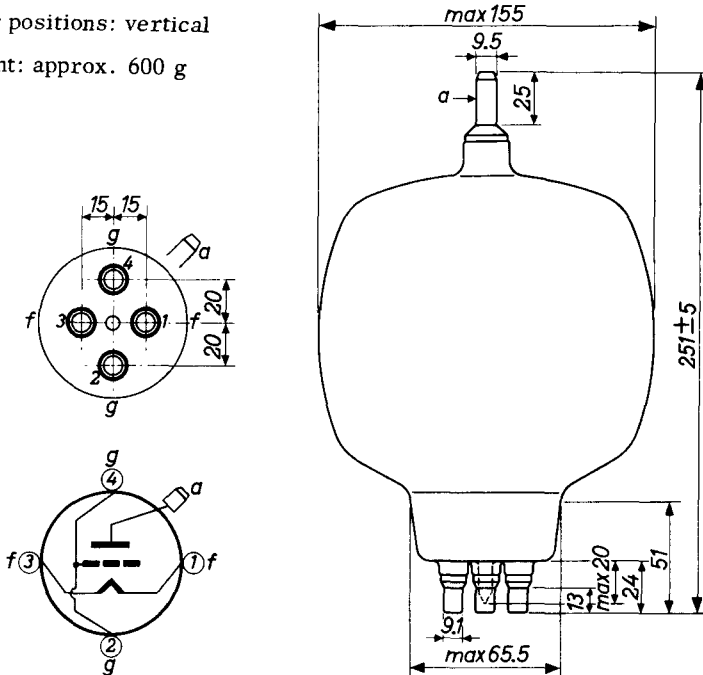
Fig. 1 Mechanical outline.
