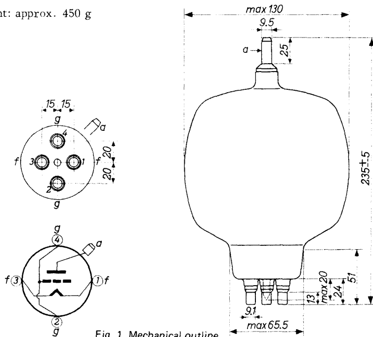
Fig. 1 Mechanical outline.
