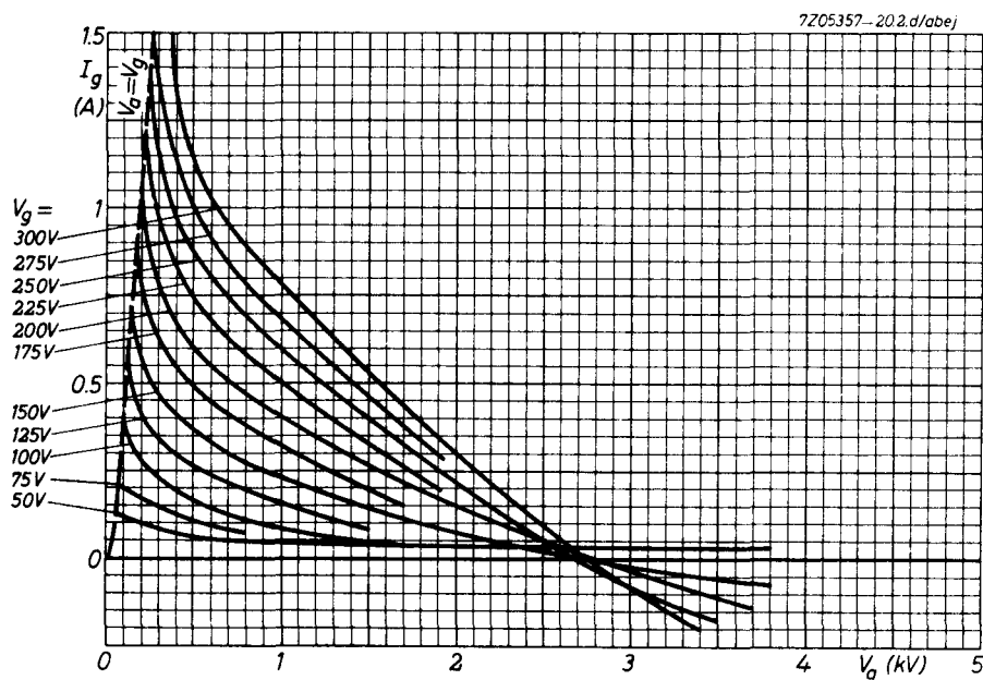
Fig. 4 I_a/V_a characteristics.
