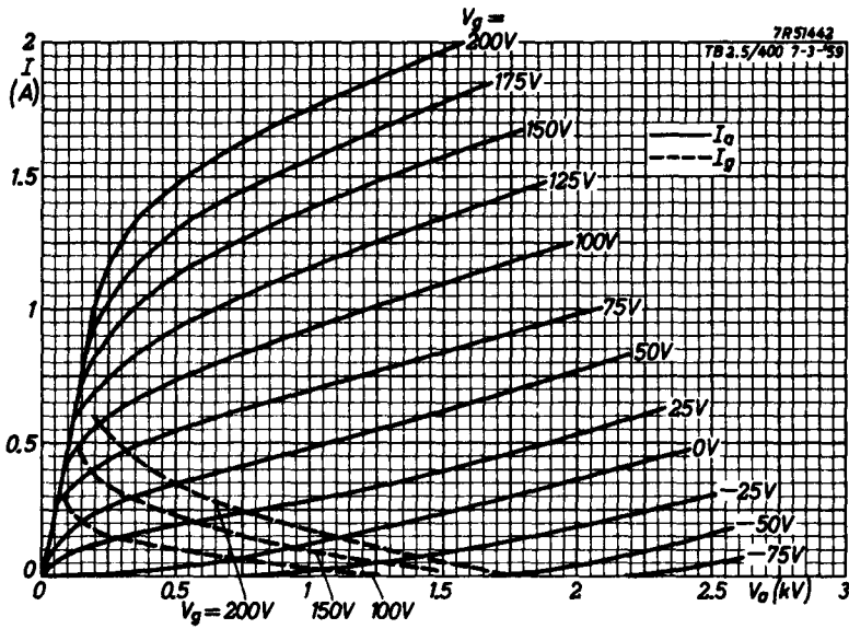
Fig. 4 I_g/V_a characteristics.
