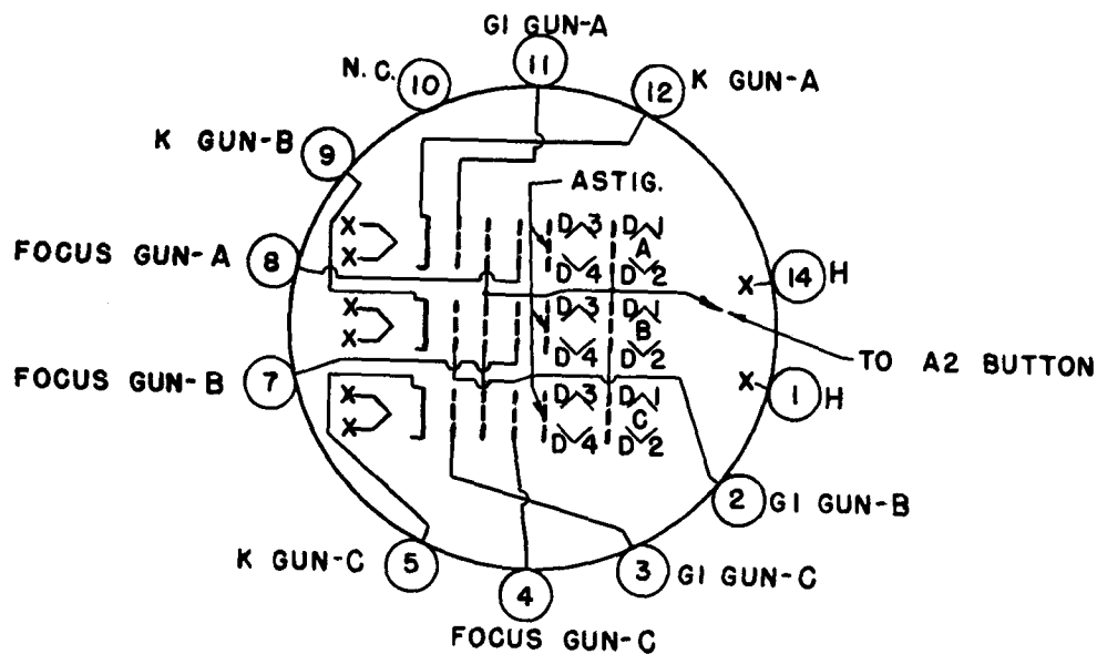
BASING DIAGRAM VIEW FROM BASE END
