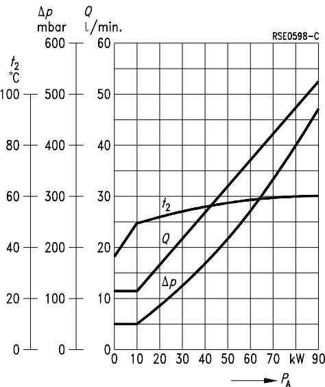
Cooling water diagram
