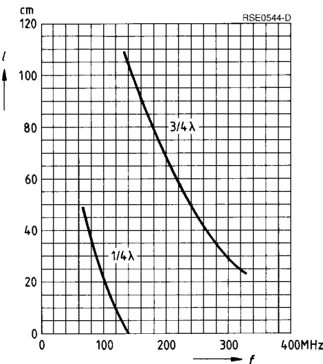
Tuning curves for coaxial circuits
