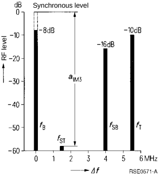
Level diagram
