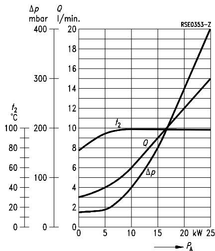
Cooling water diagram (RS 1092 SK)
