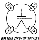
BOTTOM VIEW OF SOCKET
