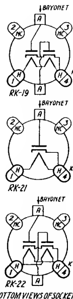
BOTTOM VIEWS OF SOCKETS
