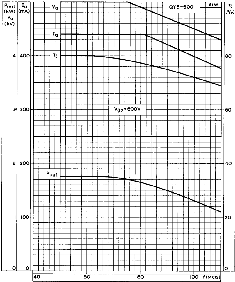
FREQUENCY CHARACTERISTICS
