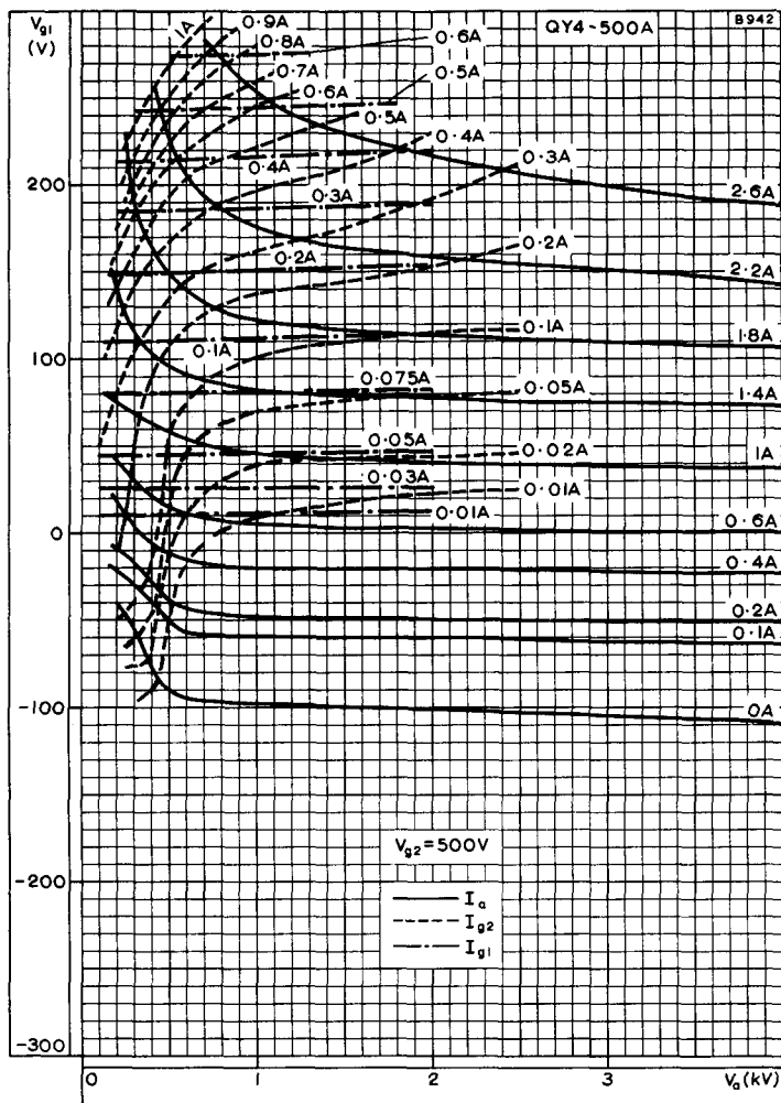
CONSTANT CURRENT CURVES V_{g2} = 500V
