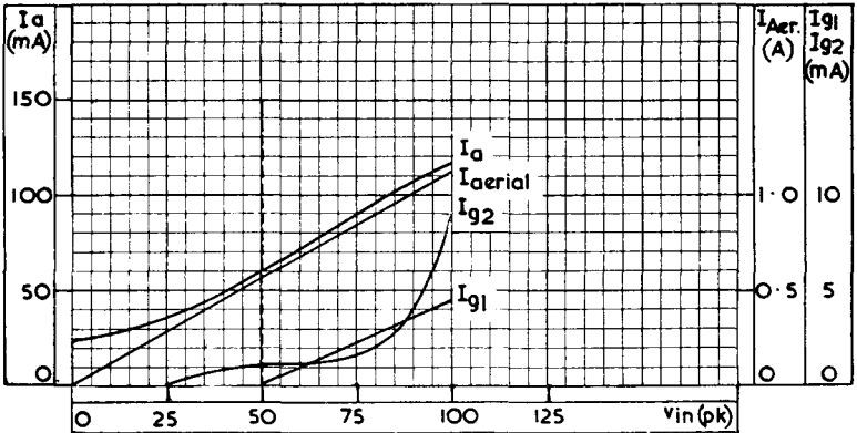
OPERATING CHARACTERISTICS FOR CLASS "B" TELEPHONY AT V_a = 3.0 kV
