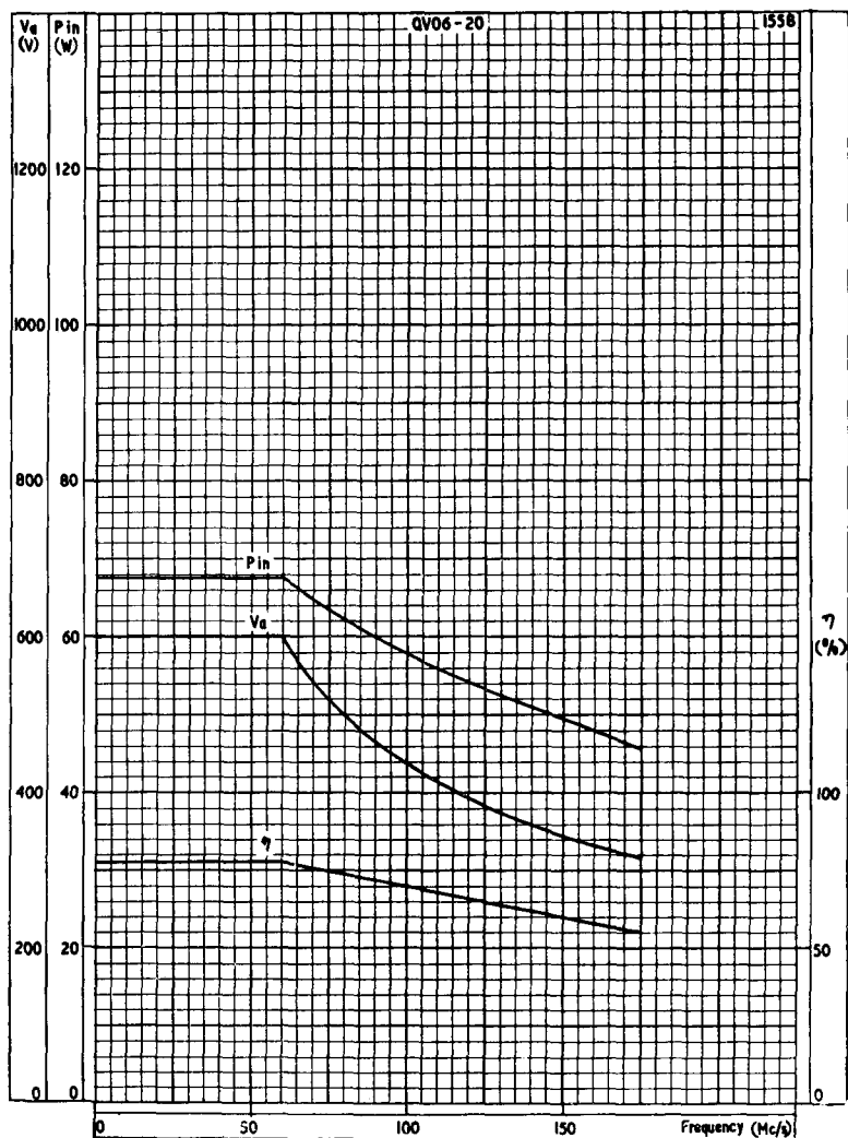
FREQUENCY CHARACTERISTICS
