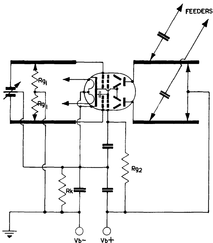
CIRCUIT DIAGRAM FOR QQQ07-40 AS V.H.F. PUSH-PULL R.F. POWER AMPLIFIER
