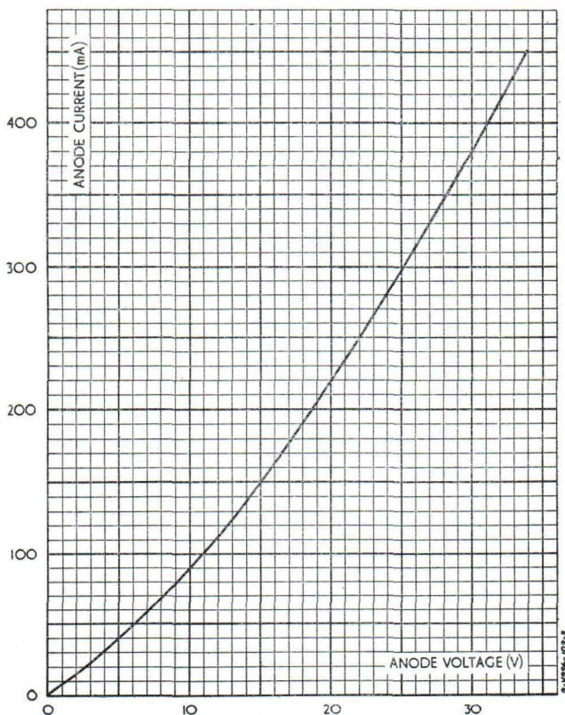
AVERAGE CHARACTERISTIC CURVE : I_a/V_a
