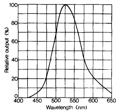
P-20 Phosphor Spectral Output
