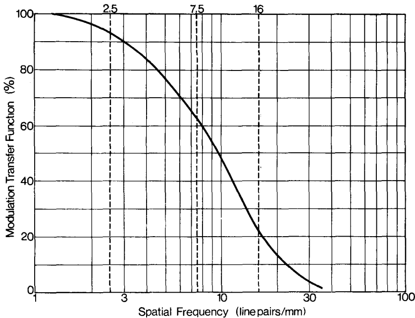
Typical Modulation Transfer Function (MTF)
