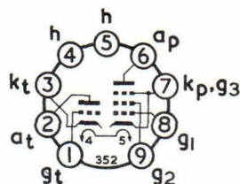
B9A Base
