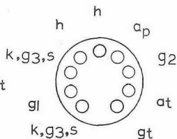
B9A Base All dimensions in mm
