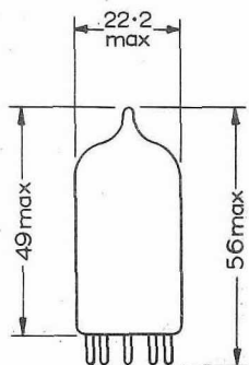
B9A Base All dimensions in mm
