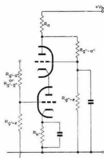
Circuit A
