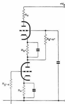
Circuit B
