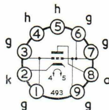
B9A Base
