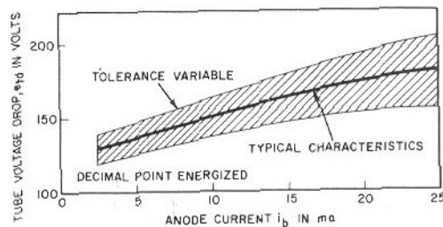
TUBE CHARACTERISTICS — STROBE
