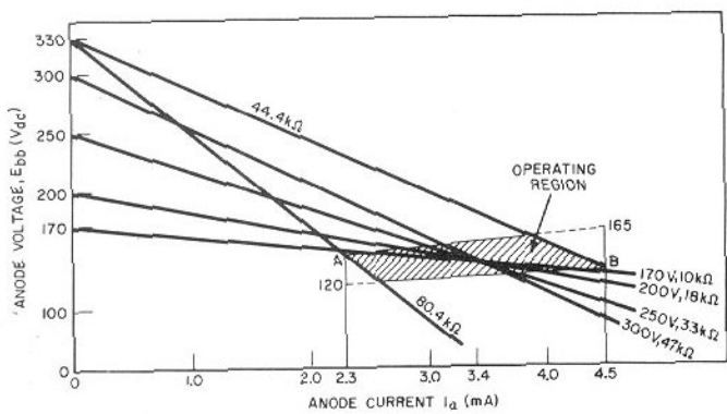
TUBE CHARACTERISTICS - dc
