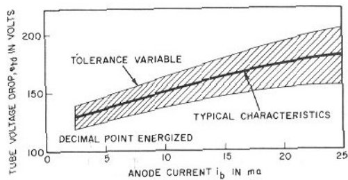
TUBE CHARACTERISTICS — STROBE
