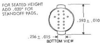
OUTLINE DRAWING
