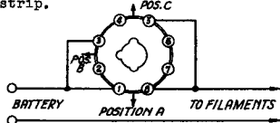
FIG. 2 BOTTOM OF SPECIAL SOCKET
