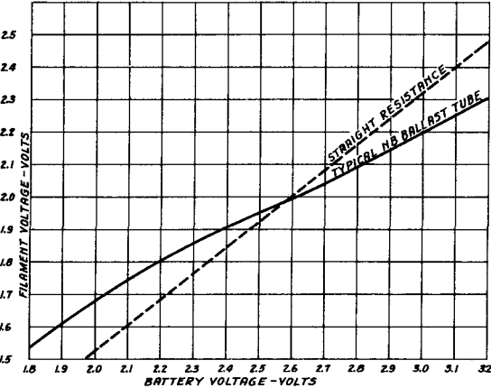
TYPICAL BALLASTING CHARACTERISTIC CURVE NB RESISTANCE TUBE 3 VOLT DRY CELL CONNECTION
