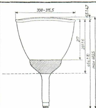
Base Culot Duodecal 9p. Sockel
