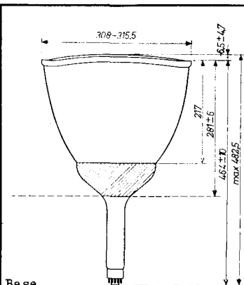
Base Culot Duodecal 7p Sockel
