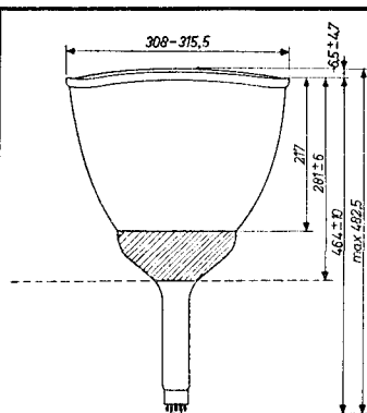
Base Culot Duodecal 7p. Sockel
