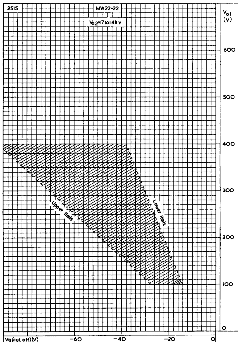
LIMITS OF GRID CUT-OFF VOLTAGE FOR FIRST ANODE VOLTAGES FROM 100 TO 400V
