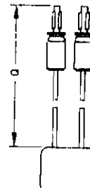
Detail of M5196B Heater and Cathode Terminals
