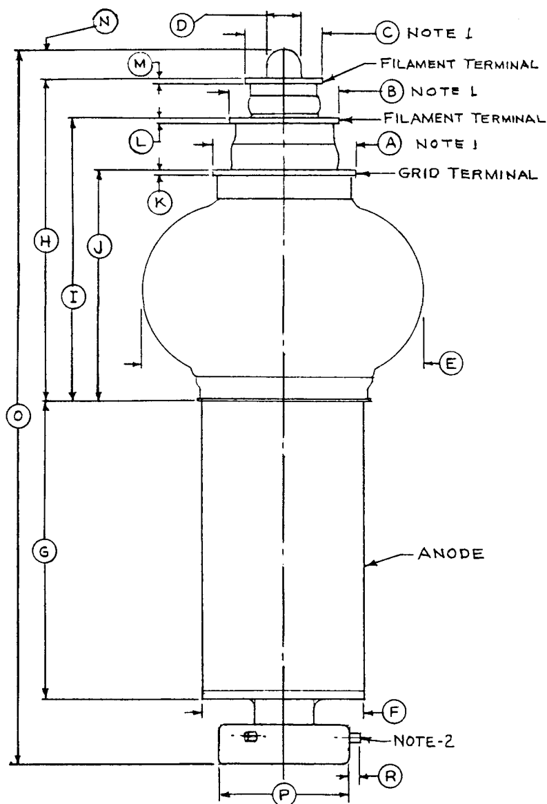
DIMENSIONS FOR OUTLINE OF ML-LPT 50
