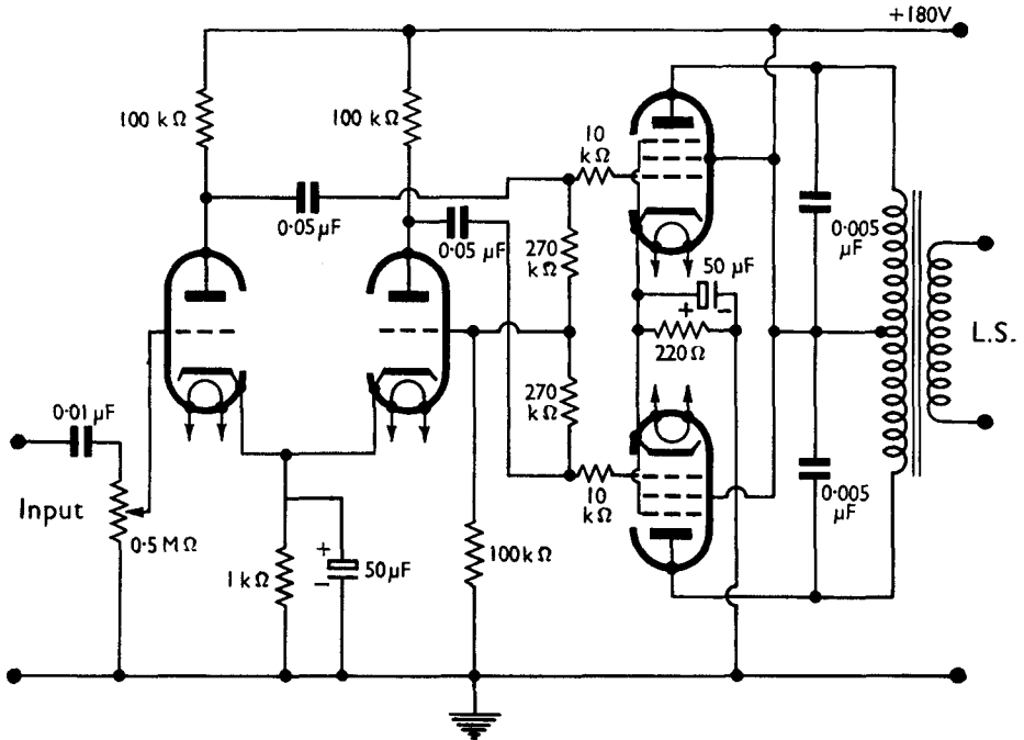
FIG. 2. Push-pull amplifier.
