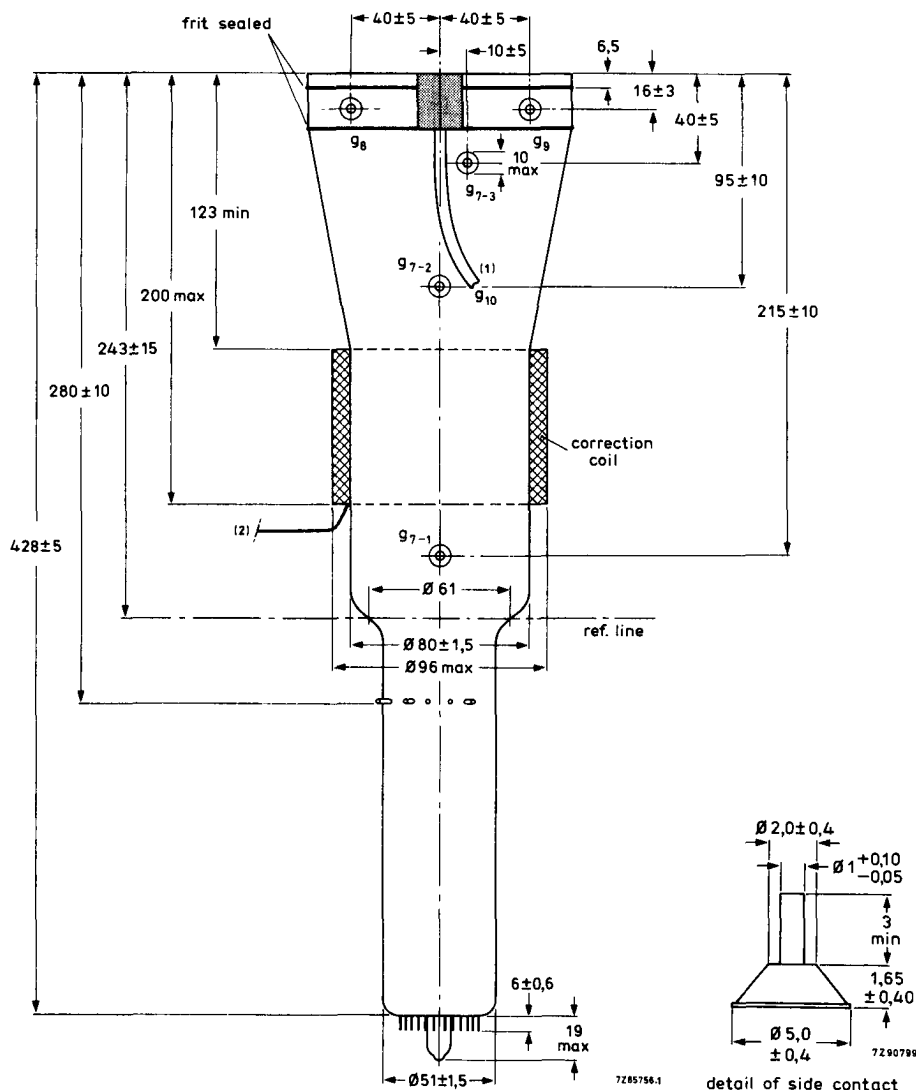
Fig. 1 Outlines.
