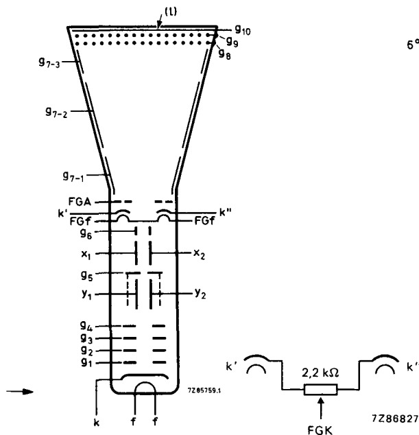
Fig. 4 Electrode configuration.
