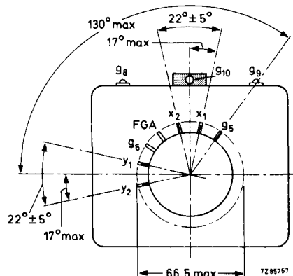
Fig. 3 Bottom view and side-contact arrangement.
