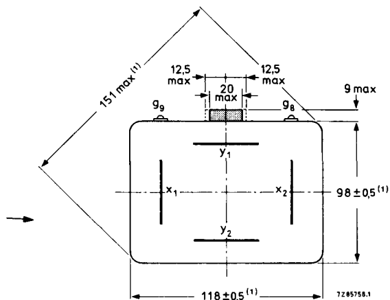
Fig. 2 Top view.
