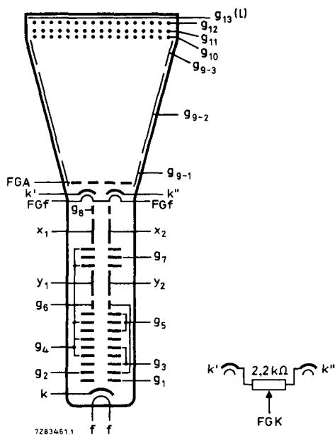
Fig. 4 Electrode configuration.
