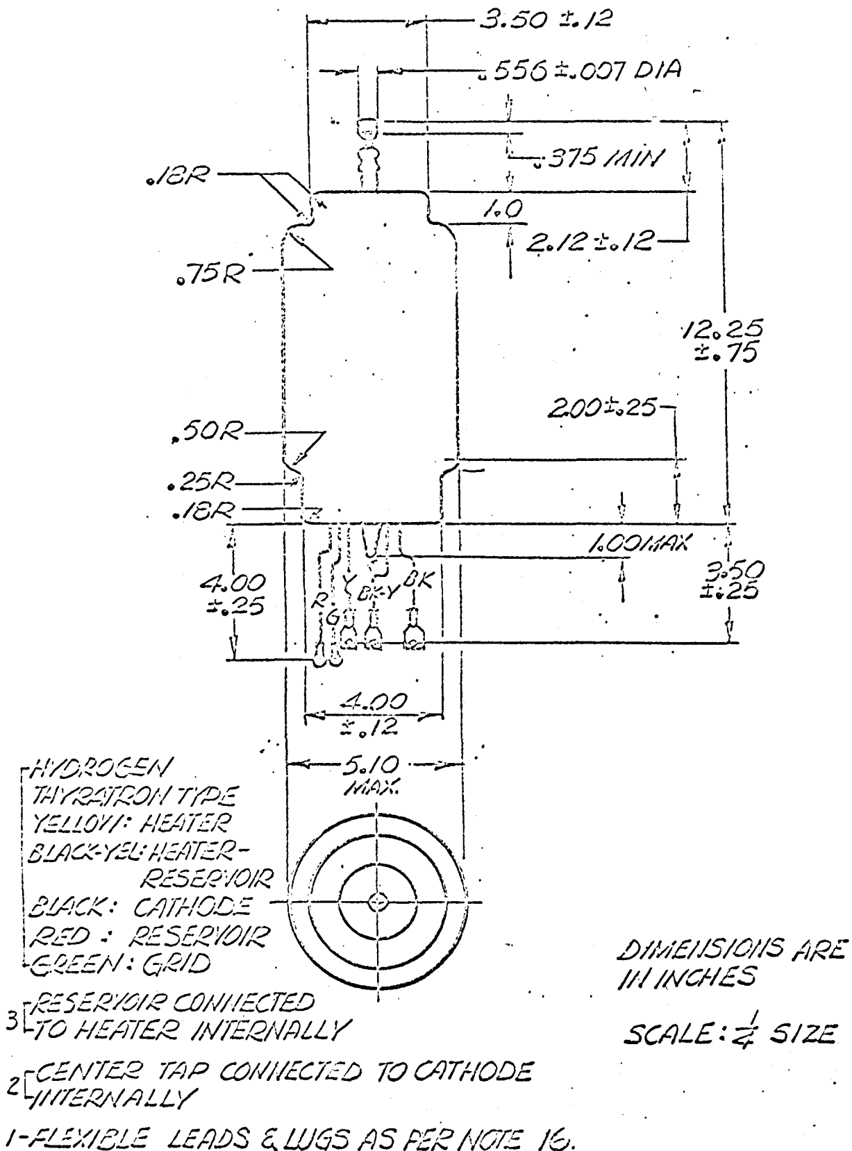
FIGURE 1. ELECTRON TUBE TYPE USAF KU-54
