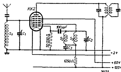
Fig. 9 The KK 2 in a short-wave circuit.
