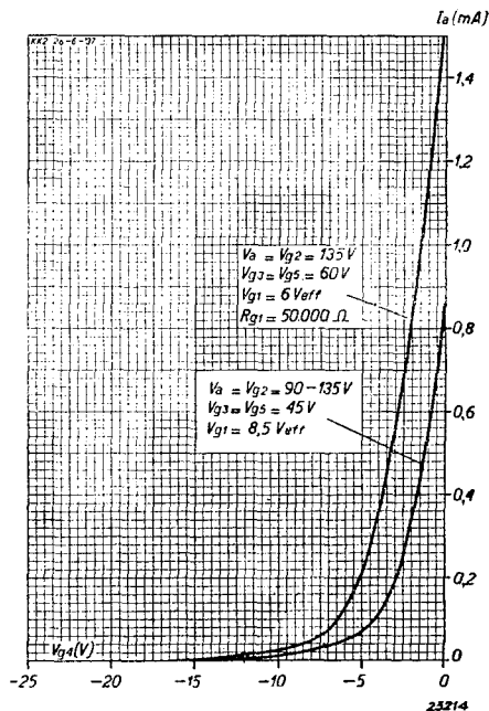
Fig. 3 Anode current as a function of the grid bias, at V_{g3,5} = 45 V and 60 V.
