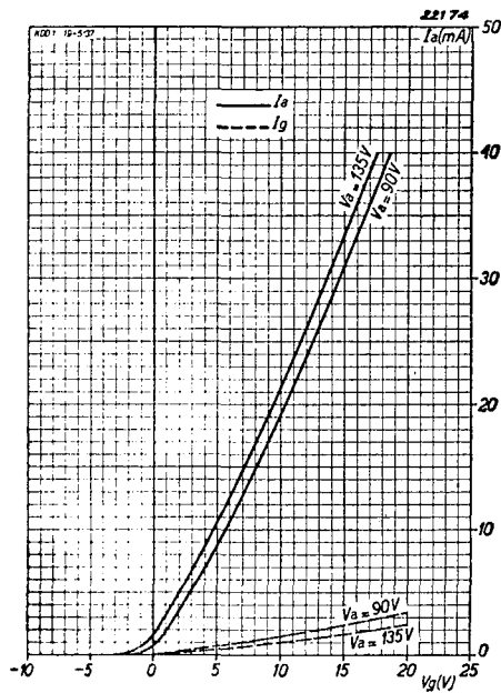
Fig. 3 Anode current and grid current as functions of the grid voltage.
