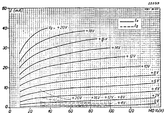
Fig. 4 Anode current and grid current as functions of the anode voltage, with grid voltage as parameter.
