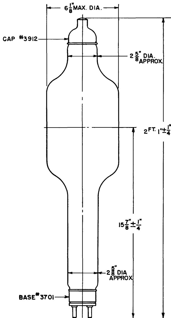
OUTLINE KC-4 KENOTRON
