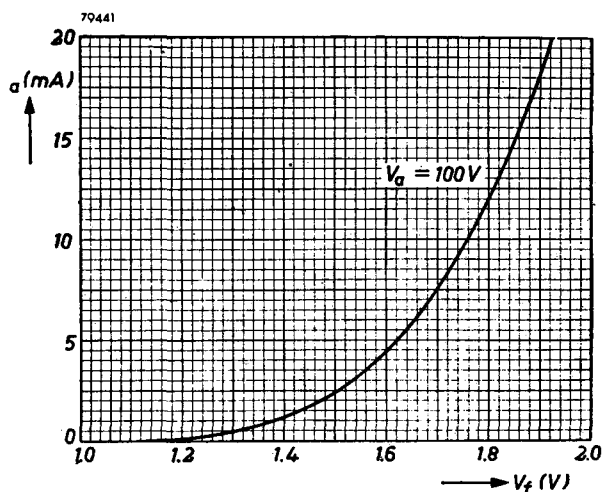
Fig. 66. I_a/V_{g1} characteristic of the K81A at an anode voltage of 100 V.
