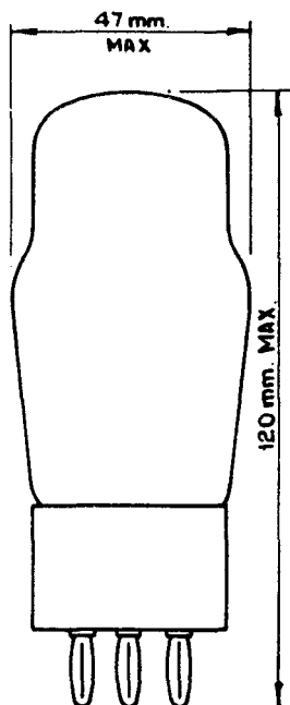
4-PIN BASE
