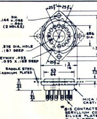
FIG. 7 HUMAN ENGINEERED NUMBER SHAPES USED ON ALL TUBE TYPES
