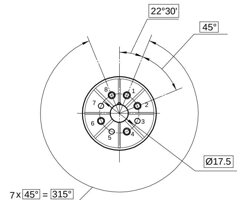
Pin arrangement
