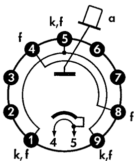
Basing diagram
