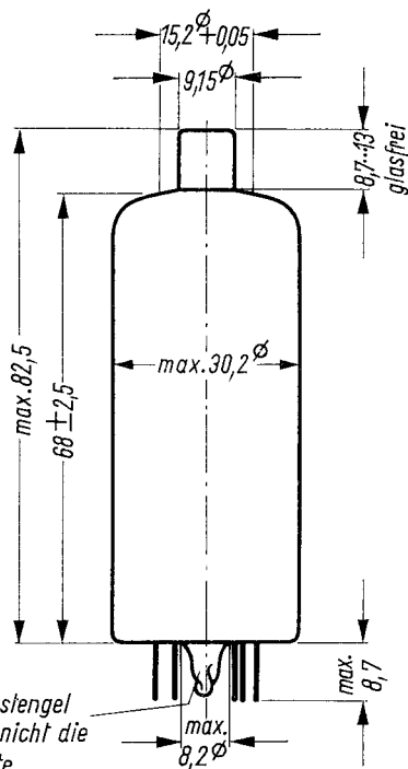
Abmessungen in mm Dimensions
