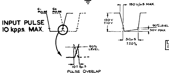
Paired-Pulse Drive
