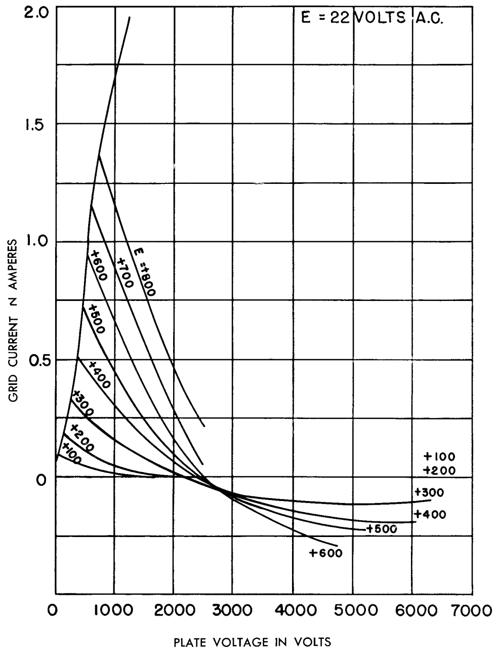
GL-891 GRID-CURRENT CHARACTERISTICS ( E_i = 22 VOLTS A-C)
