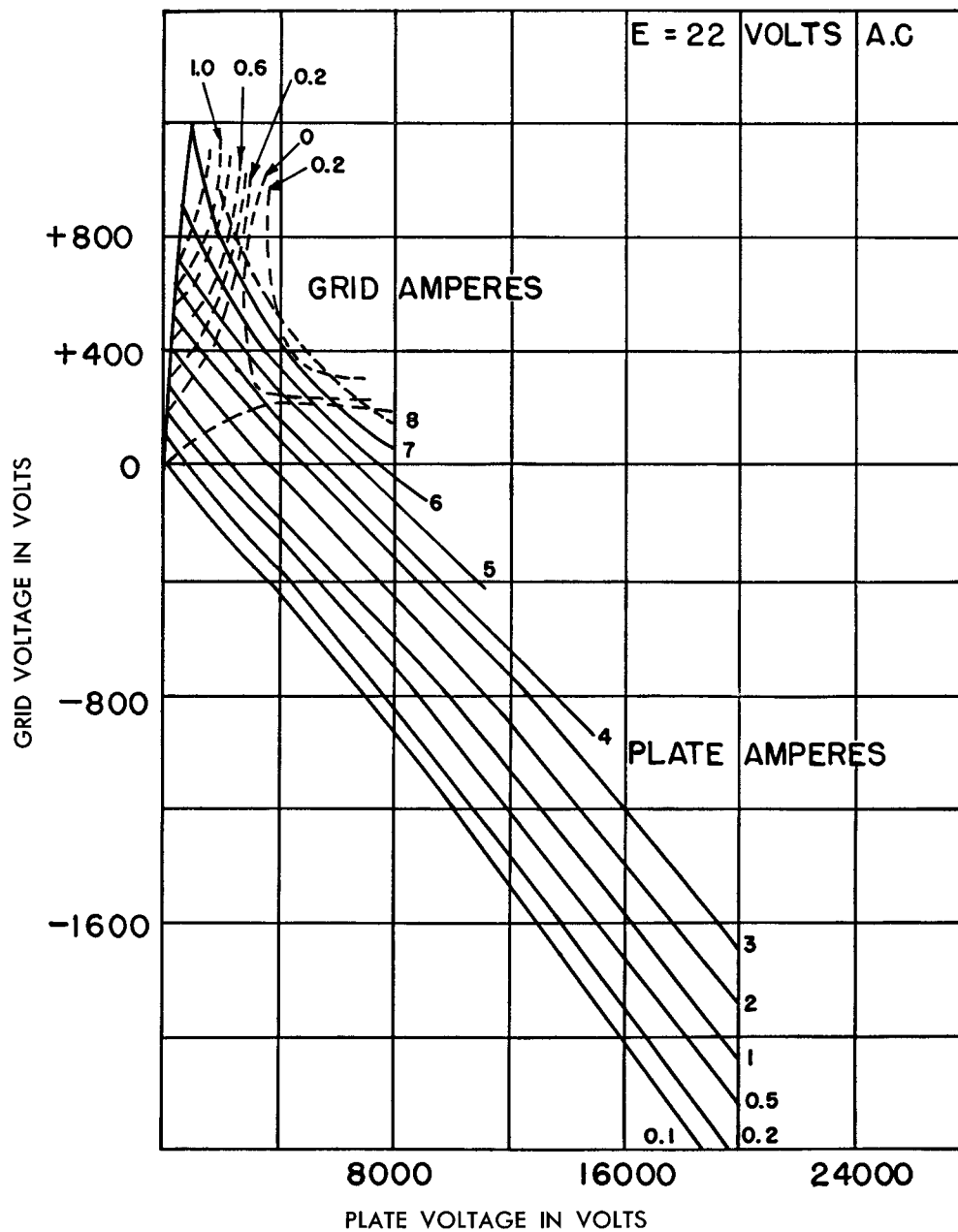
GL-891 CONSTANT CURRENT PLATE AND GRID CHARACTERISTICS ( E_g = 22 VOLTS A-C)
