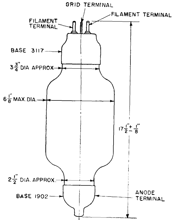
OUTLINE GL-851 PIOTRON
