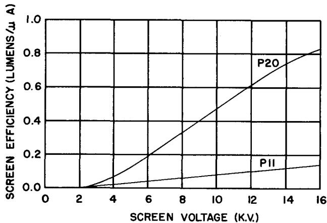
FIGURE 3 TYPICAL LUMINOUS EFFICIENCY OF P11 AND P20
