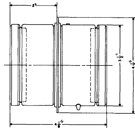
FIGURE 4 OUTLINE DRAWING
