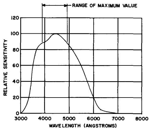
FIGURE 1 S11 SPECTRAL RESPONSE
