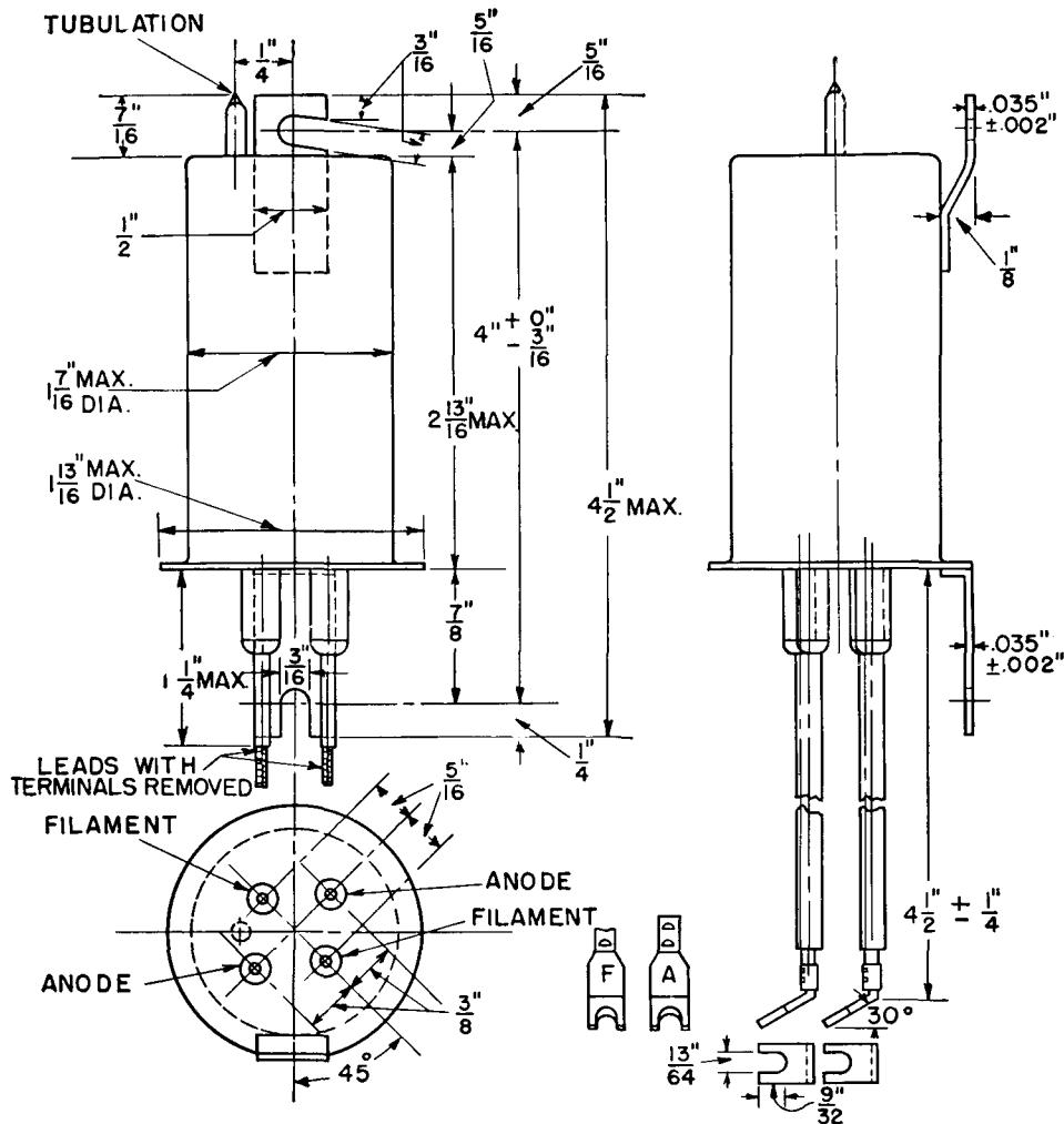
OUTLINE FG-190 PHANOTRON
